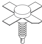
CASE 145D-02 STYLE 1 (.380" SOE)
